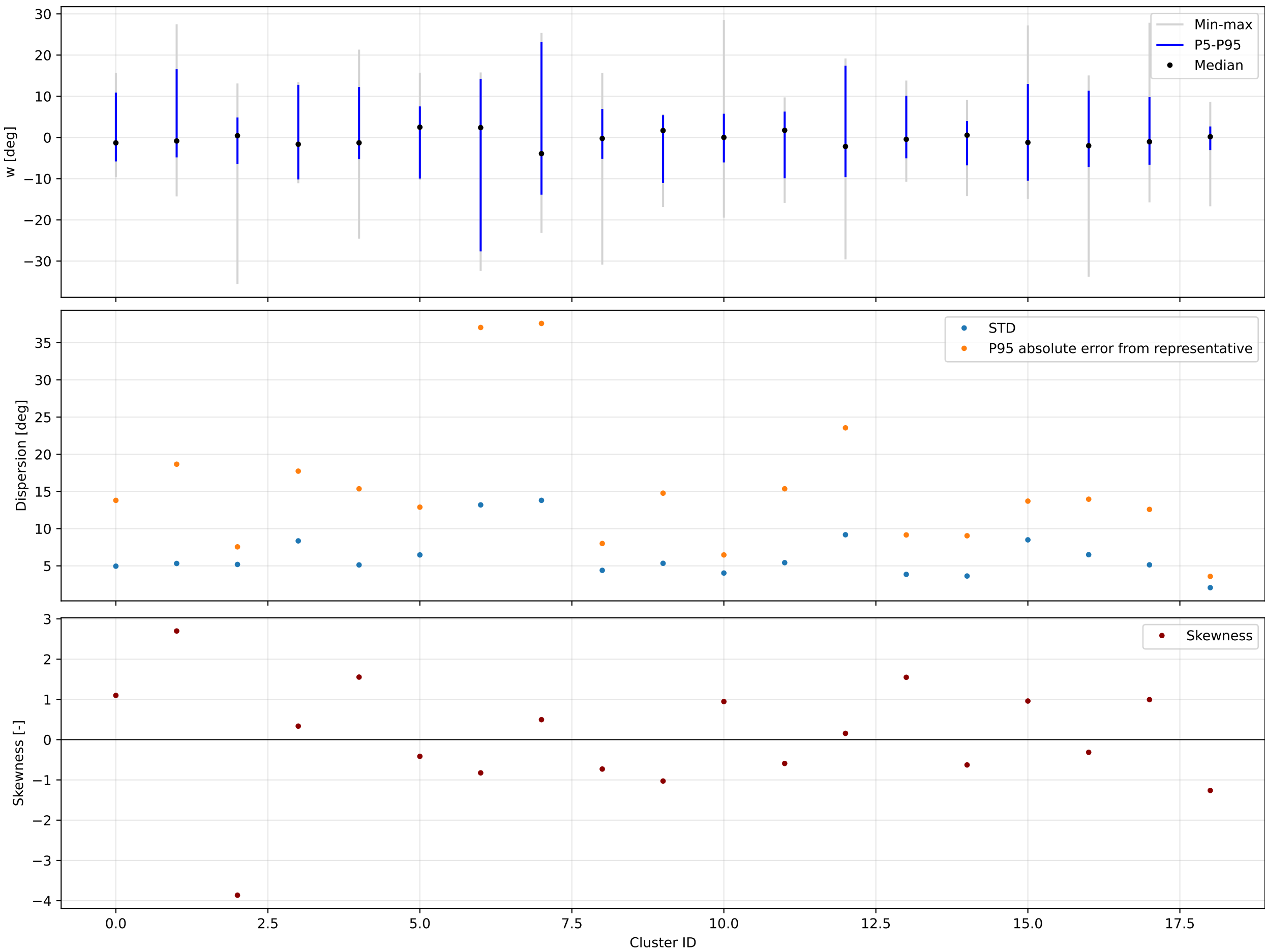
K=19 | backward | w | valid=194124/194124 | offsets from each cluster circular mean
