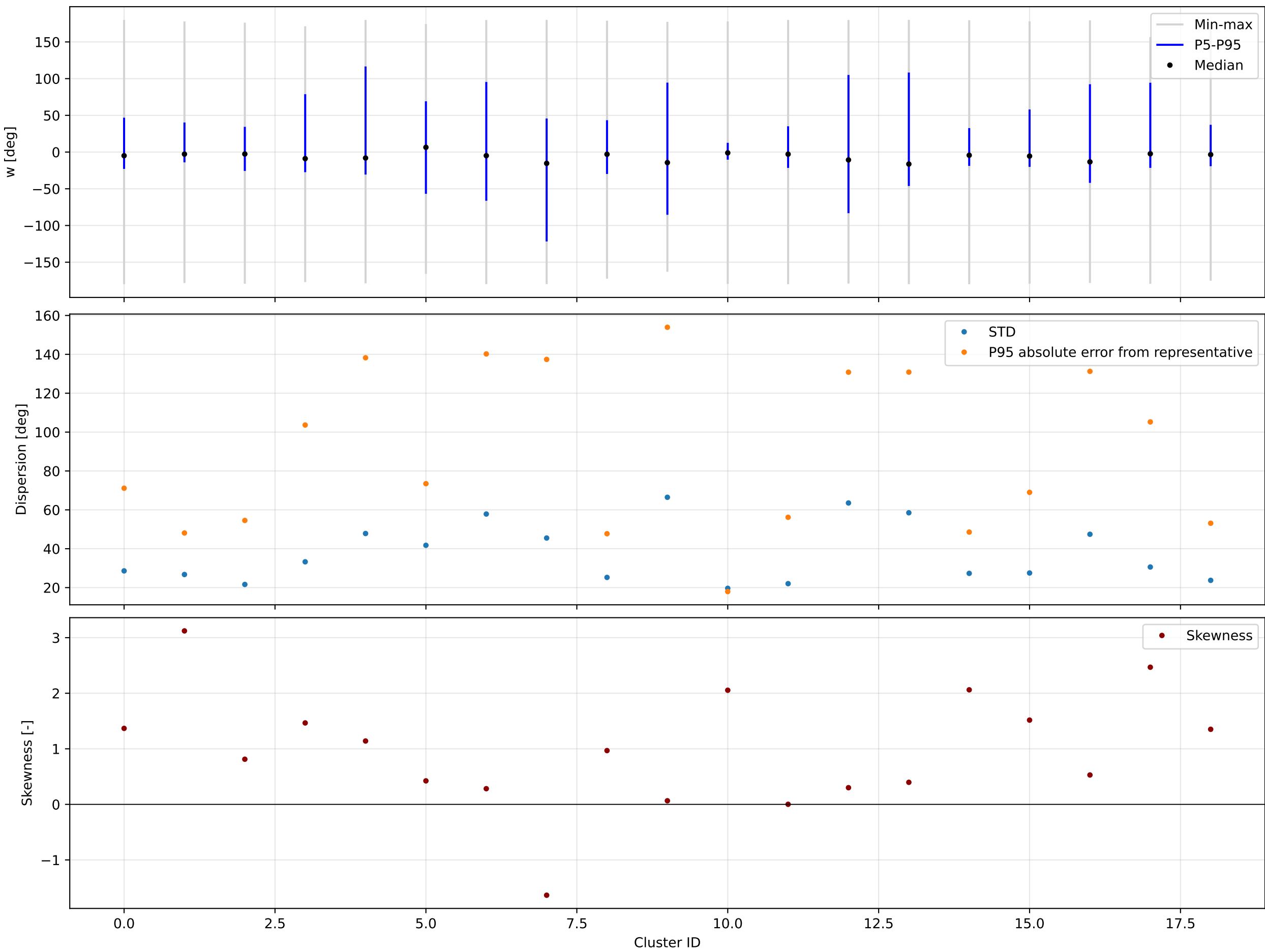
K=19 | forward | w | valid=194058/194124 | offsets from each cluster circular mean
